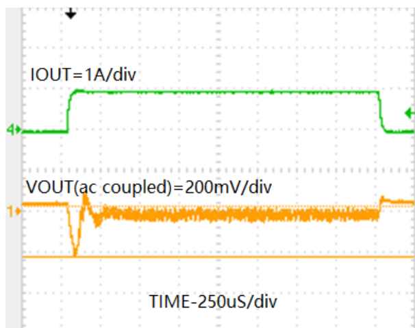
阶跃负载(PVIN=3.7V, VOUT=9V, IOUT=0 to 1A)
