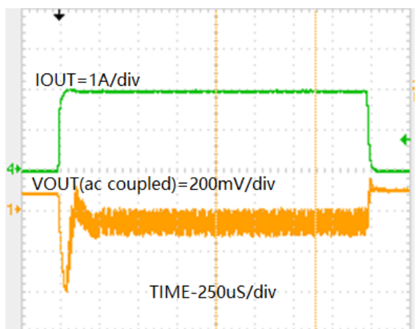
阶跃负载(PVIN=7.4V, VOUT=15V, IOUT=0 to 2A)
