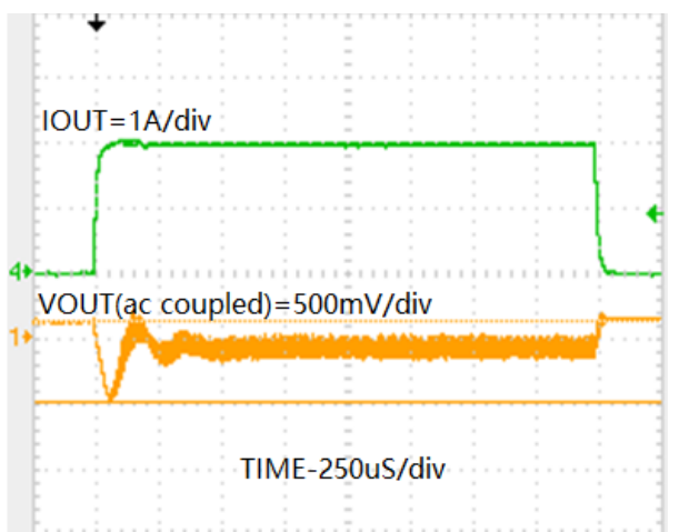
阶跃负载(PVIN=7.4V, VOUT=18V, IOUT=0. to 2A)
