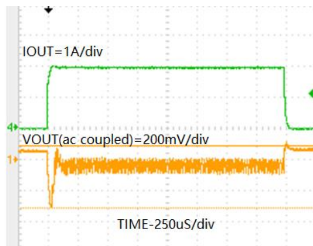
阶跃负载(PVIN=7.4V, VOUT=12V, IOUT=0. to 2A)
